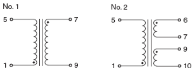
Circuit Diagram
