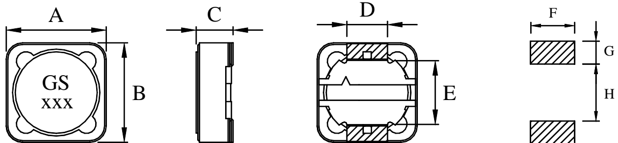
Land Pattern
